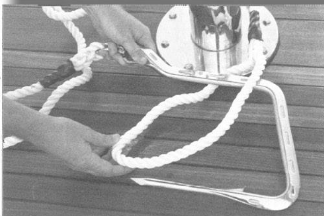
Above: Before you attach the flying gaff head to the pole, make sure the tail end of the rope is secured to an anchor point on the boat. The gamechair post is ideal.
